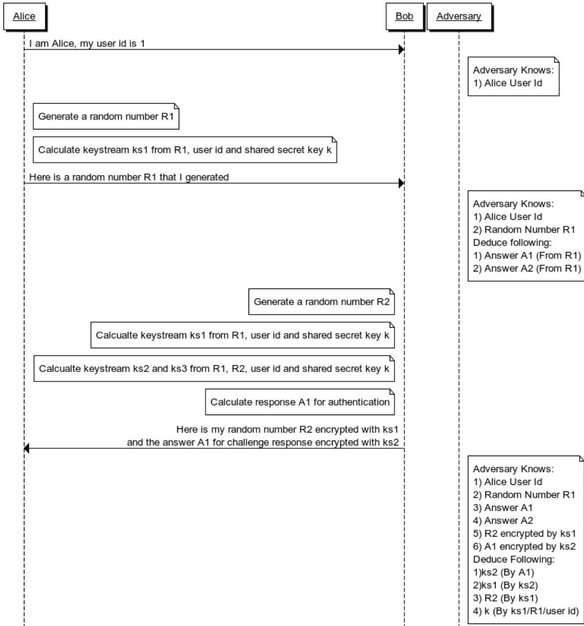
Figure 3 Simple Authentication Sequence Example
