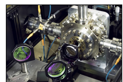
Accelerator Science
