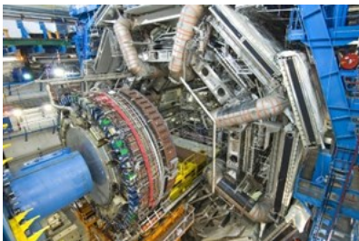
Particle Physics
