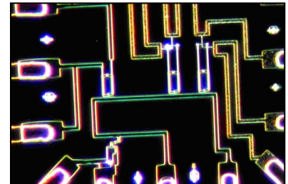
Nanophysics
